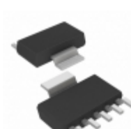
MCP1826T-0802E/DC Microchip Technology IC REG LDO 0.8V 1A SOT223-5
