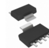
MCP1826T-1202E/DC Microchip Technology IC REG LDO 1.2V 1A SOT223-5
