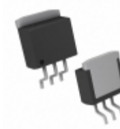
MIC2940A-5.0BU Microchip Technology IC REG LDO 5V 1.25A TO263-3
