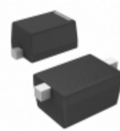
CMOZ210 TR Central Semiconductor Corp DIODE ZENER 2V 250MW SOD523
