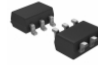
S-1721A1825-M6T1G SII Semiconductor Corporation IC REG LIN 1.8V/2.5V 0.15A SOT23
