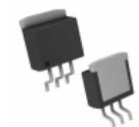
MIC2940A-12BU TR Microchip Technology IC REG LDO 12V 1.25A TO263-3
