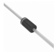
1N4764A B0G TSC (Taiwan Semiconductor) DIODE ZENER 100V 1W DO204AL
