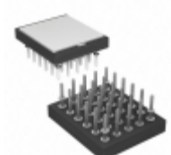
AT28C010-15UM/883 Microchip Technology IC EEPROM 1MBIT 150NS 30CPGA
