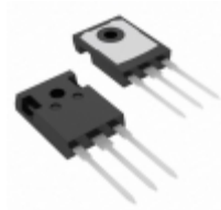
FGH25N120FTDS Fairchild/ON Semiconductor IGBT 1200V 50A 313W TO247
