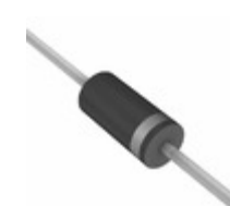
BZW06-85 R0G TSC (Taiwan Semiconductor) TVS DIODE 85.5V 178V DO204AC
