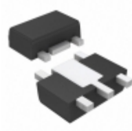
AP2112R5A-2.5TRG1 Diodes Incorporated IC REG LDO 2.5V 0.6A
