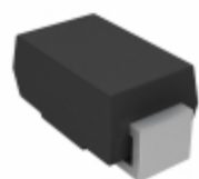
US1G-M3/5AT Vishay Semiconductor Diodes Division DIODE 1A 400V 50NS DO-214AC
