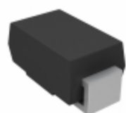
US1G-M3/61T Vishay Semiconductor Diodes Division DIODE 1A 400V 50NS DO-214AC
