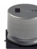
EEV-TG1E102M Panasonic Electronic Components CAP ALUM 1000UF 20% 25V SMD
