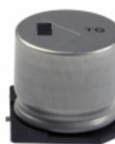
EEV-TG1K471M Panasonic Electronic Components CAP ALUM 470UF 20% 80V SMD
