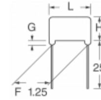
ECQ-P4474JU Panasonic Electronic Components CAP FILM 0.47UF 5% 400VDC RADIAL
