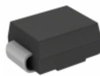
SMBJ60CA Littelfuse Inc. TVS DIODE 60VWM 96.8VC SMB
