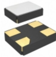
CX3225SB19200H0FLJCC AVX Corporation CRYSTAL 19.2000MHZ 12PF SMD
