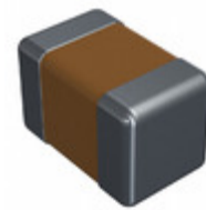
CDR31BP120BJWSAP Electro-Films (EFI) / Vishay CAP CER 12PF 100V BP 0805
