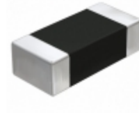
QVS107CG3R9CCHT Taiyo Yuden CAP CER 3.9PF 250V NP0 0603
