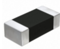
QVS107CG560JCHT Taiyo Yuden CAP CER 56PF 250V NP0 0603
