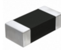
QVS107CG4R7BCHT Taiyo Yuden CAP CER 4.7PF 250V NP0 0603
