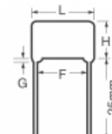
ECQ-P1H682GZ3 Panasonic Electronic Components CAP FILM 6800PF 2% 50VDC RADIAL
