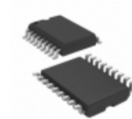
PIC16C715-20I/SO Microchip Technology IC MCU 8BIT 3.5KB OTP 18SOIC
