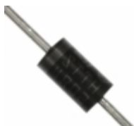
STTH4R02 STMicroelectronics DIODE GEN PURP 200V 4A DO201AB
