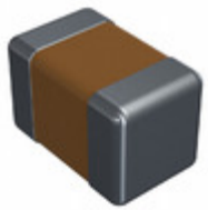
CDR31BP101BKWRAP Electro-Films (EFI) / Vishay CAP CER 100PF 100V BP 0805
