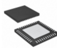
PIC24FJ64GA004-I/ML Microchip Technology IC MCU 16BIT 64KB FLASH 44QFN
