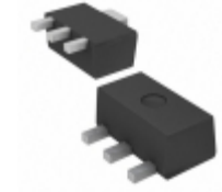
AP130-25YL-13 Diodes Incorporated IC REG LDO 2.5V 0.3A SOT89-3
