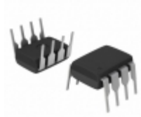
MCP4911-E/P Microchip Technology DAC 10BIT SGL W/SPI 8DIP
