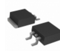
VS-8EWH06FNTRHM3 Electro-Films (EFI) / Vishay DIODE GEN PURP 600V 8A D-PAK
