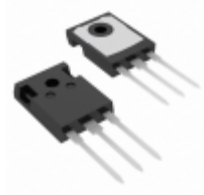
FDH44N50 Fairchild/ON Semiconductor MOSFET N-CH 500V 44A TO-247
