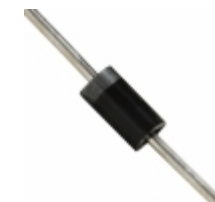
1N4760A BK Central Semiconductor Corp DIODE ZENER 68V 1W DO41
