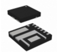
RT7238CGQUF Richtek IC REG BUCK 5.1V 8A SYNC 10UQFN
