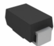
SMBZ5929B-E3/5B Vishay Semiconductor Diodes Division DIODE ZENER 15V 3W DO214AA
