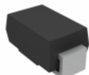
SMBZ5929B-E3/52 Vishay Semiconductor Diodes Division DIODE ZENER 15V 3W DO214AA
