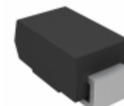
SMBZ5928B-E3/5B Vishay Semiconductor Diodes Division DIODE ZENER 13V 3W DO214AA
