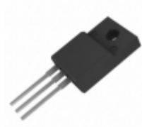
AOTF20S60L Alpha and Omega Semiconductor, Inc. MOSFET N-CH 600V 20A TO220F
