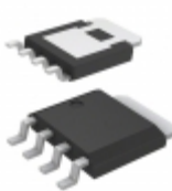
BUK7Y41-80EX Nexperia USA Inc. MOSFET N-CH 80V 25A LPAK
