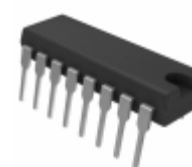
ADM8697AN Analog Devices Inc. IC SUPERVSR MPU ADJ/RESET 16DIP
