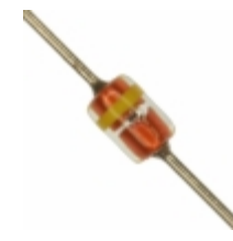
MTZJT-7213C Rohm Semiconductor DIODE ZENER 13V 500MW DO34
