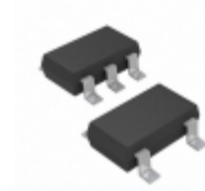
MIC5256-2.85BD5-TR Microchip Technology IC REG LDO 2.85V 0.15A TSOT23-5
