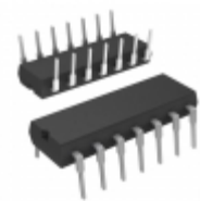
MM74HC86N AMI Semiconductor / ON Semiconductor IC GATE XOR 4CH 2-INP 14DIP
