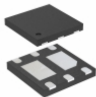
AON2810 Alpha & Omega Semiconductor Inc. MOSFET 2N-CH 30V 2A 6DFN
