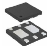
AON2812 Alpha & Omega Semiconductor Inc. MOSFET 2N-CH 30V 4.5A
