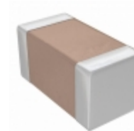
C1005C0G1H151J/50 TDK Corporation CAP CER 150PF 50V C0G 0402
