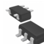
XC6121C330MR-G Torex Semiconductor Ltd IC WATCHDOG TIMER SOT-25
