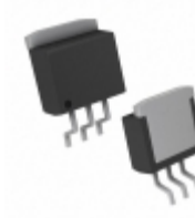
MIC5237-5.0BU Microchip Technology IC REG LDO 5V 0.5A TO263-3
