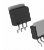
MIC5237-3.3BU TR Microchip Technology IC REG LDO 3.3V 0.5A TO263-3
