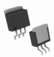
MIC2937A-3.3WU-TR Microchip Technology IC REG LDO 3.3V 0.75A TO263-3
