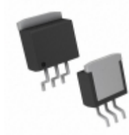
MIC2937A-3.3BU TR Microchip Technology IC REG LDO 3.3V 0.75A TO263-3
