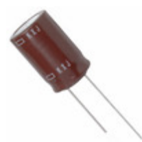
EKXJ451ELL820MU50S United Chemi-Con CAP ALUM 82UF 20% 450V RADIAL
