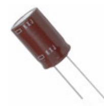
EKXJ451ETS560MM25S United Chemi-Con CAP ALUM 56UF 20% 450V RADIAL
