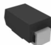
SML4753AHE3/61 Vishay Semiconductor Diodes Division DIODE ZENER 36V 1W DO214AC
