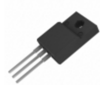
SBRF1060CTL SMC Diode Solutions DIODE SCHOTTKY 60V ITO220AB
