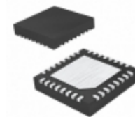
PIC24EP64MC202-E/MM Microchip Technology IC MCU 16BIT 64KB FLASH 28QFN
