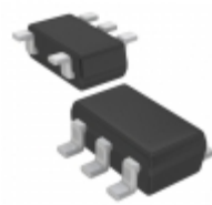
TC1017-2.8VLTTR Microchip Technology IC REG LDO 2.8V 0.15A SC70-5
