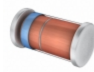
CLL4740A BK Central Semiconductor Corp DIODE ZENER 10V 1W MELF
