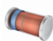
CLL4744A TR Central Semiconductor Corp DIODE ZENER 15V 1W MELF
