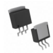
MCP1827S-1202E/EB Microchip Technology IC REG LDO 1.2V 1.5A 3DDPAK
