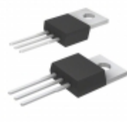
MCP1827S-1802E/AB Microchip Technology IC REG LDO 1.8V 1.5A TO220-3
