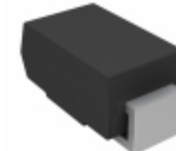
P4SMA91A-E3/61 Vishay Semiconductor Diodes Division TVS DIODE 77.8VWM 125VC SMA
