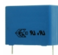
B32924E3565M EPCOS (TDK) CAP FILM 5.6UF 20% 305VAC RADIAL
