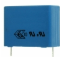
B32924E3825M EPCOS (TDK) CAP FILM 8.2UF 20% 305VAC RADIAL
